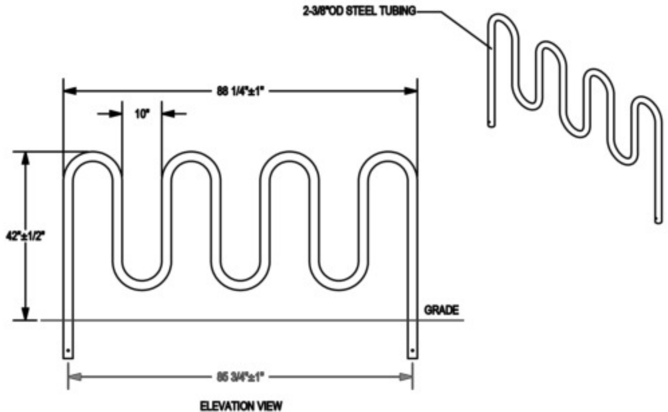
ELEVATION VIEW
