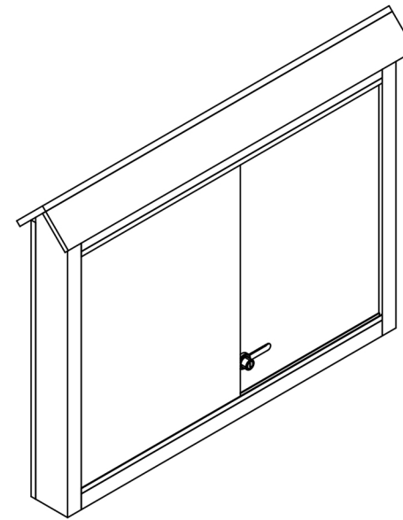
3D ISOMETRIC VIEW
