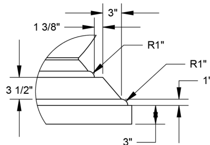
DETAIL B SCALE 1 : 12
